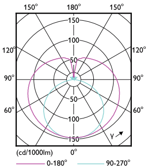
Light Distribution Diagram - Ledtube DE 1200mm 19W 830 T8 G13 EG
